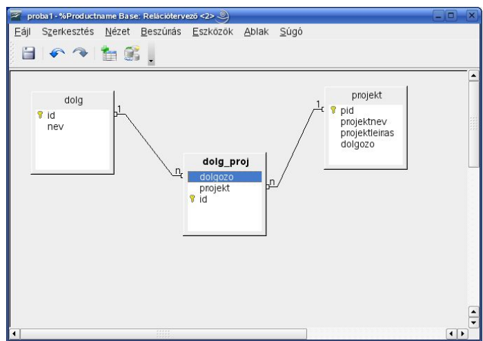
Picture 3. Relation constructor
